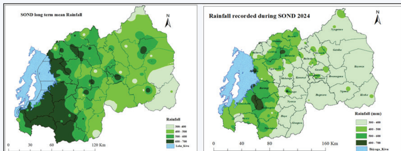
Figure 21: Long Term Average for SOND Vs Observed rainfall
