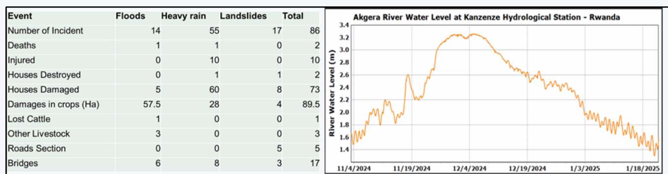
Figure 22: Reported impacts of hydrological disasters and Observed Akagera River levels in OND 2024
