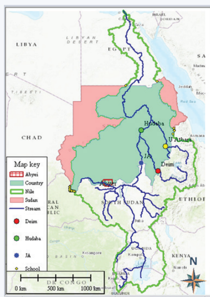
Figure 28: Sudan Nile Basin
