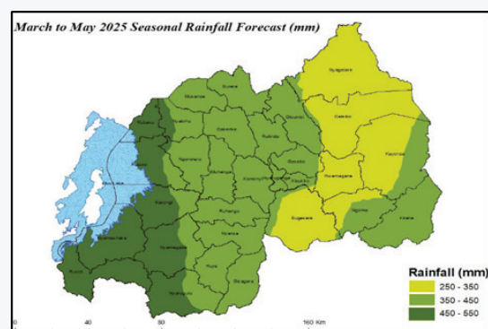
Figure 23: MAM seasonal rainfall forecast for Rwanda
