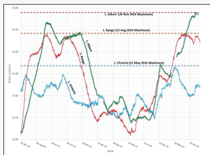
Figure 35: Observed historical lake levels in NEL region
