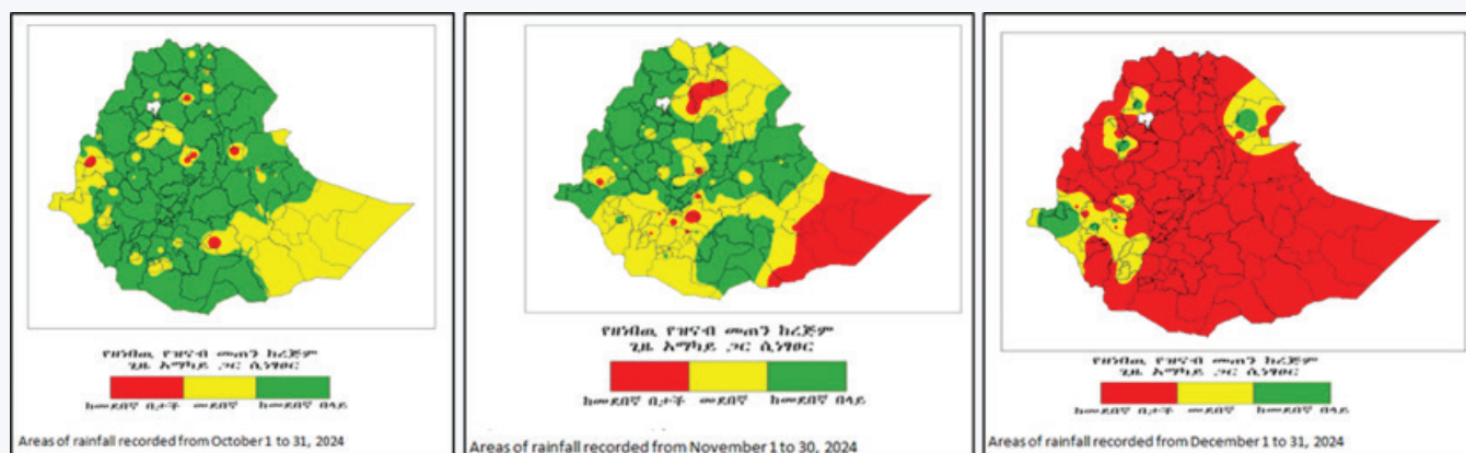
Figure 17: Recorded rainfall in OND 2024 in Ethiopia (Source: EMI)
