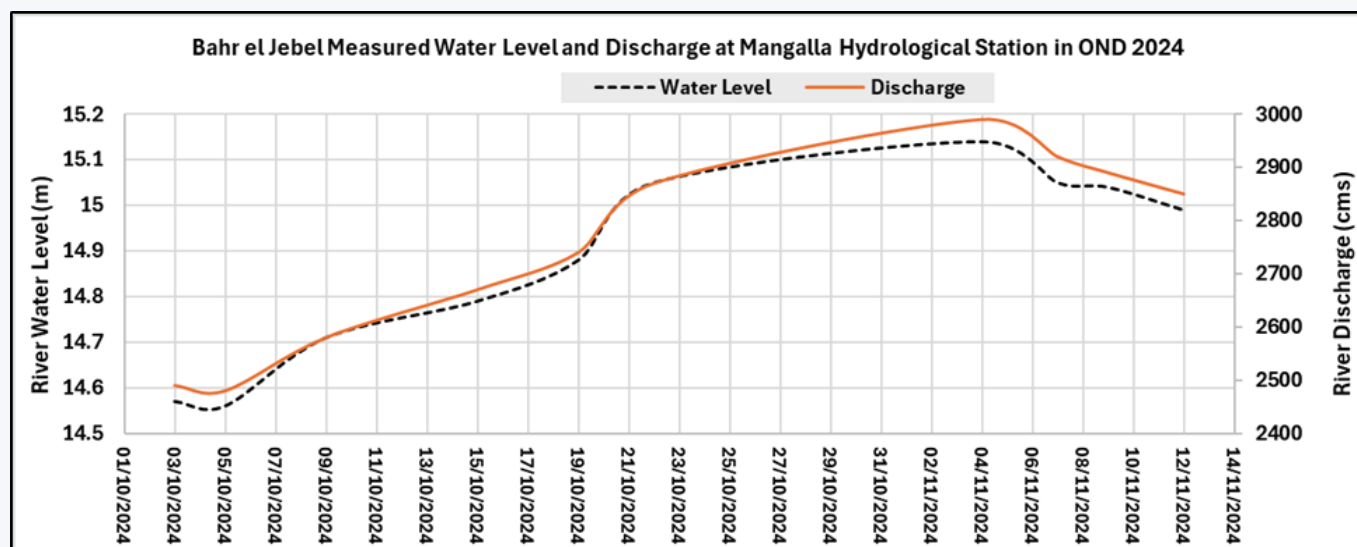
Figure 26: Daily discharge measurement on Bahr el Jebel River at Mangalla hydrological station
