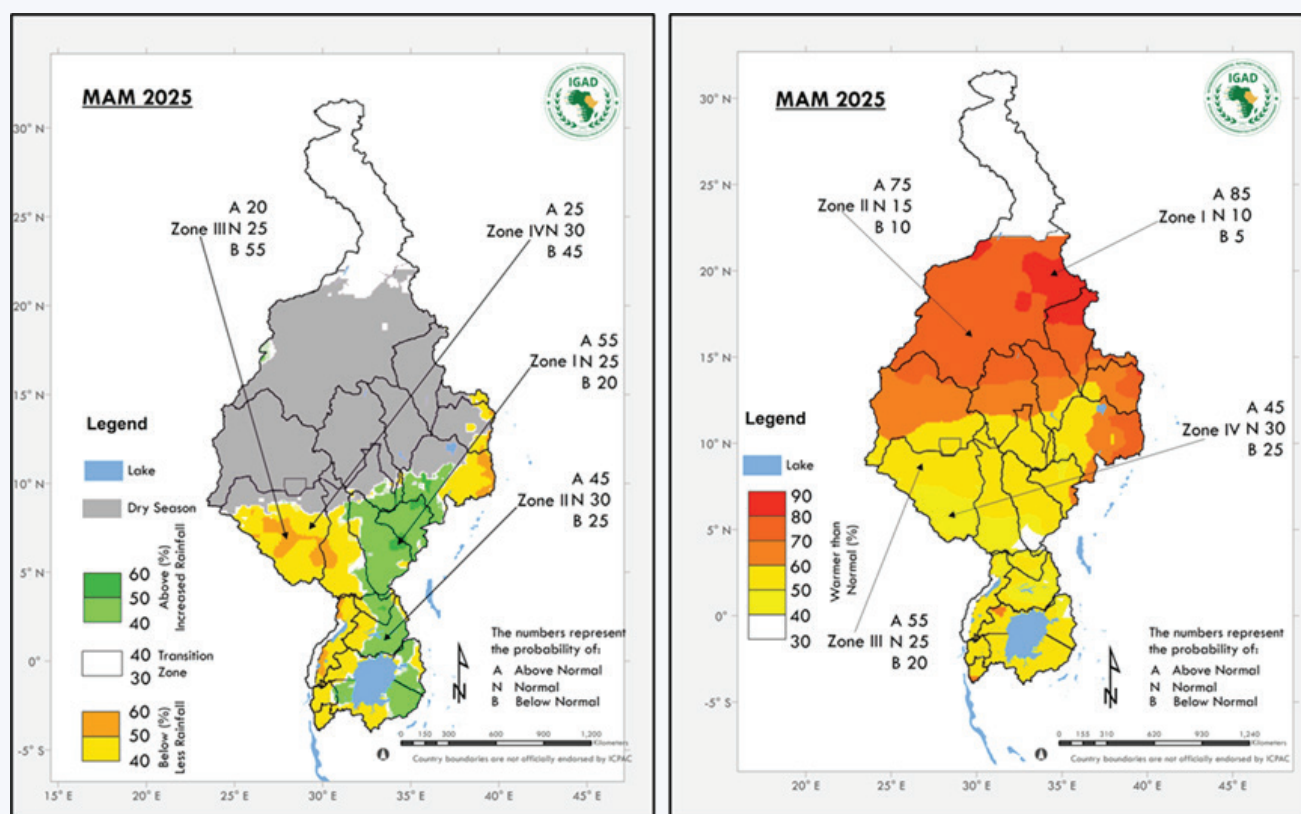
Figure 7: Nile Basin Climate Outlook for MAM 2025- Rainfall and Temperature.
