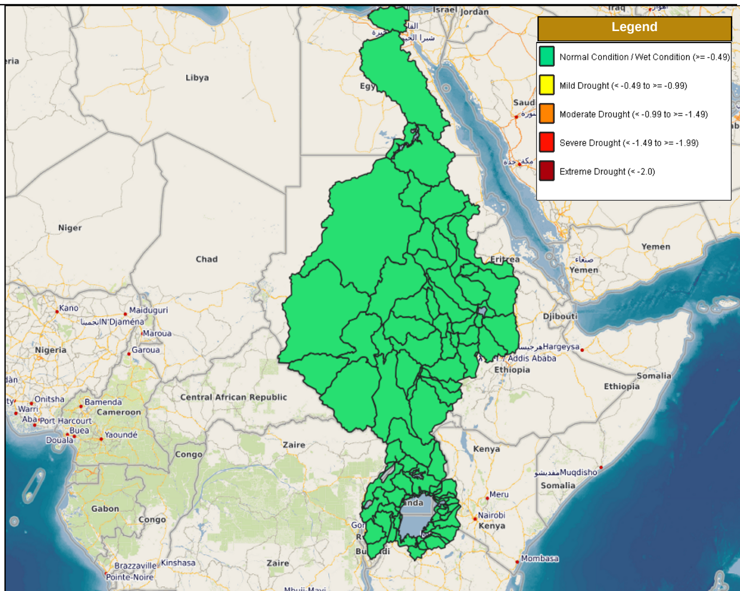
Figure 13: Spatial distribution pattern of SMAPI during the period from April 2025
