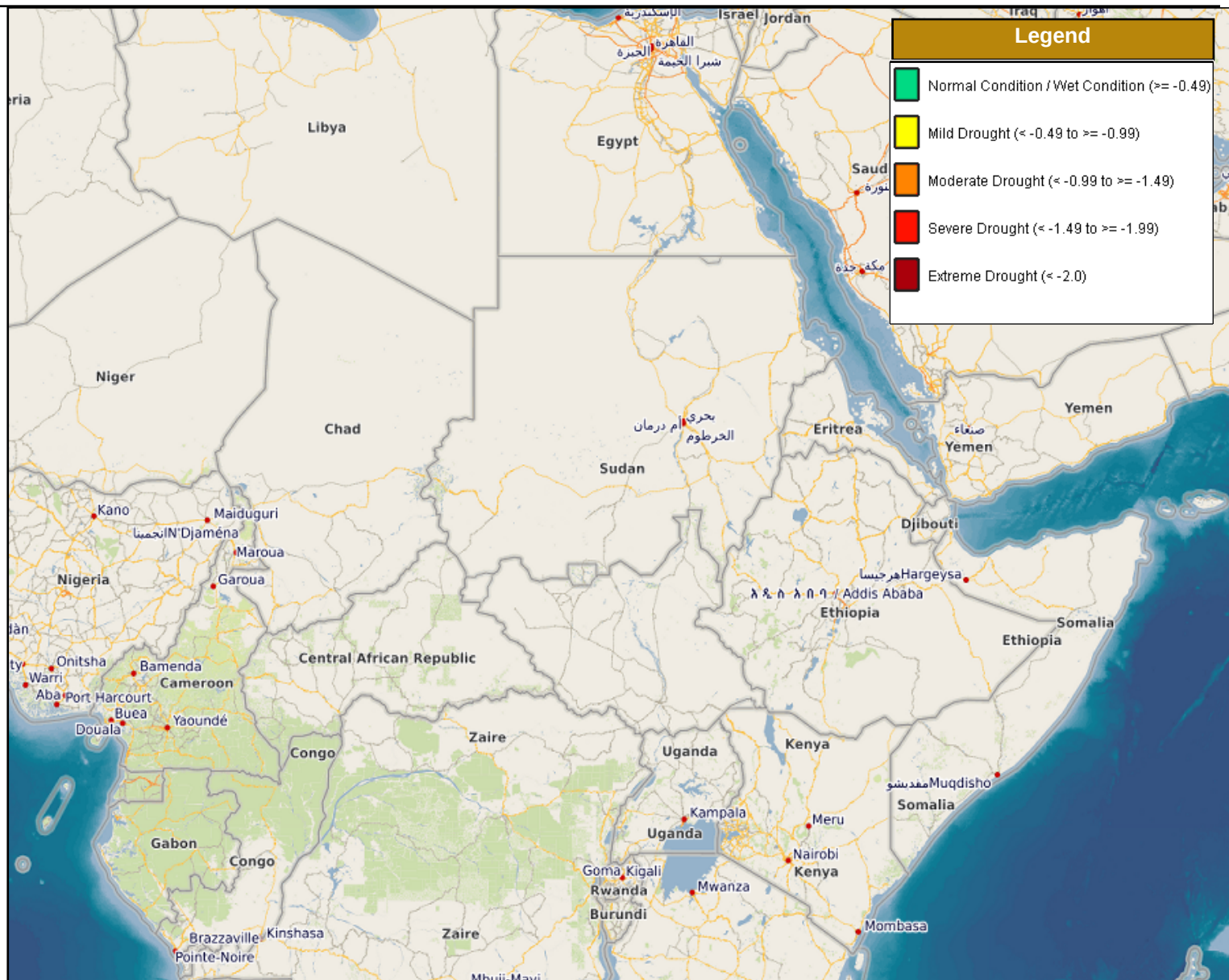
Figure 12: Spatial distribution pattern of SMAPI during the period from (16 - 30) Apr 2025
