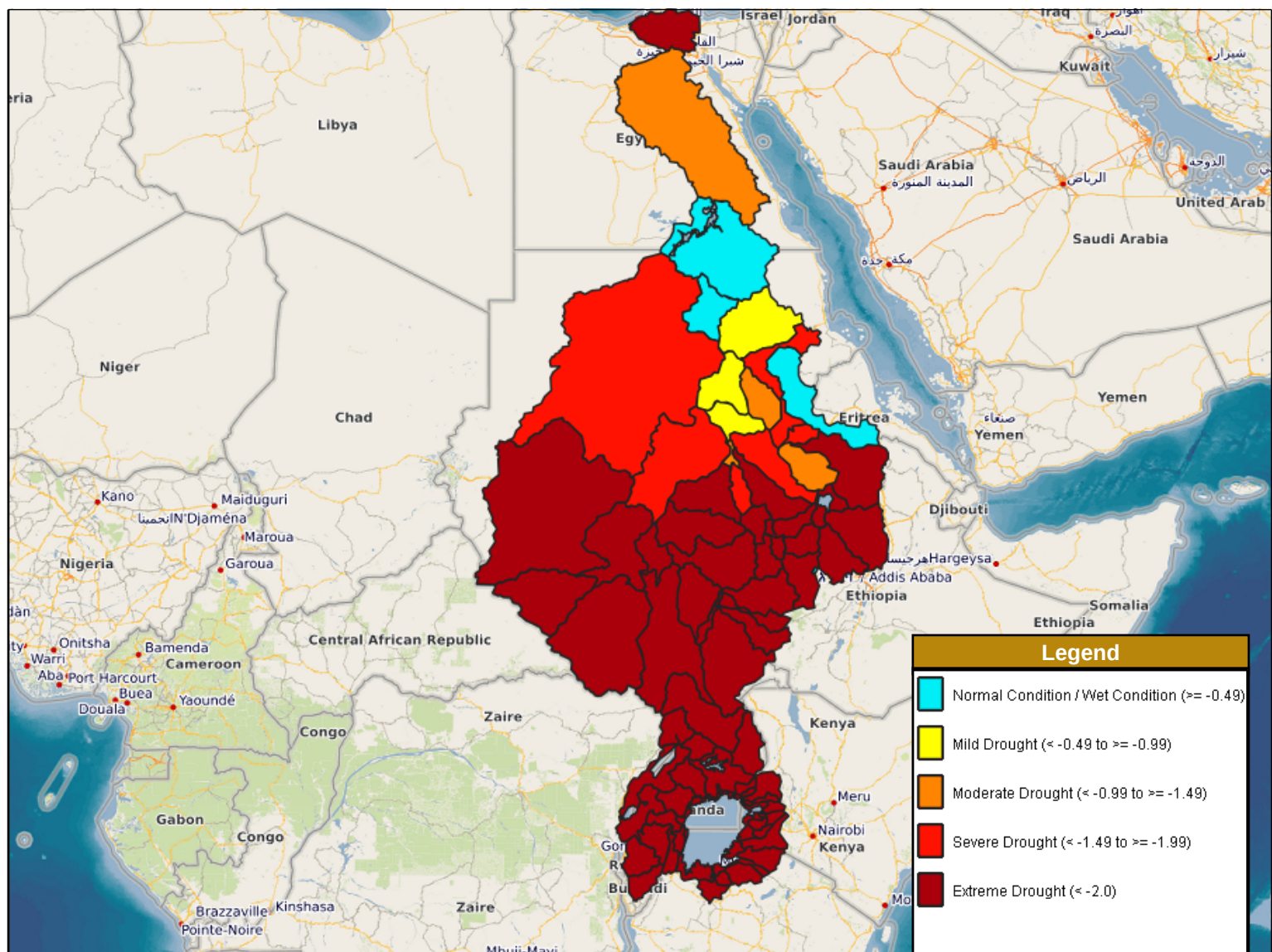
Figure 2: Spatial distribution pattern of SPI during the period from April 2025
