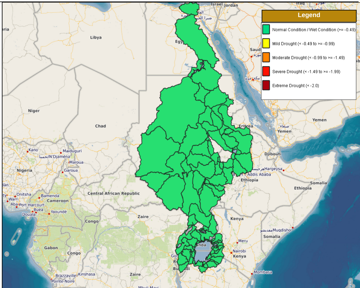
Figure 14: Spatial distribution pattern of SMAPI during the period from February-2025-April-2025
