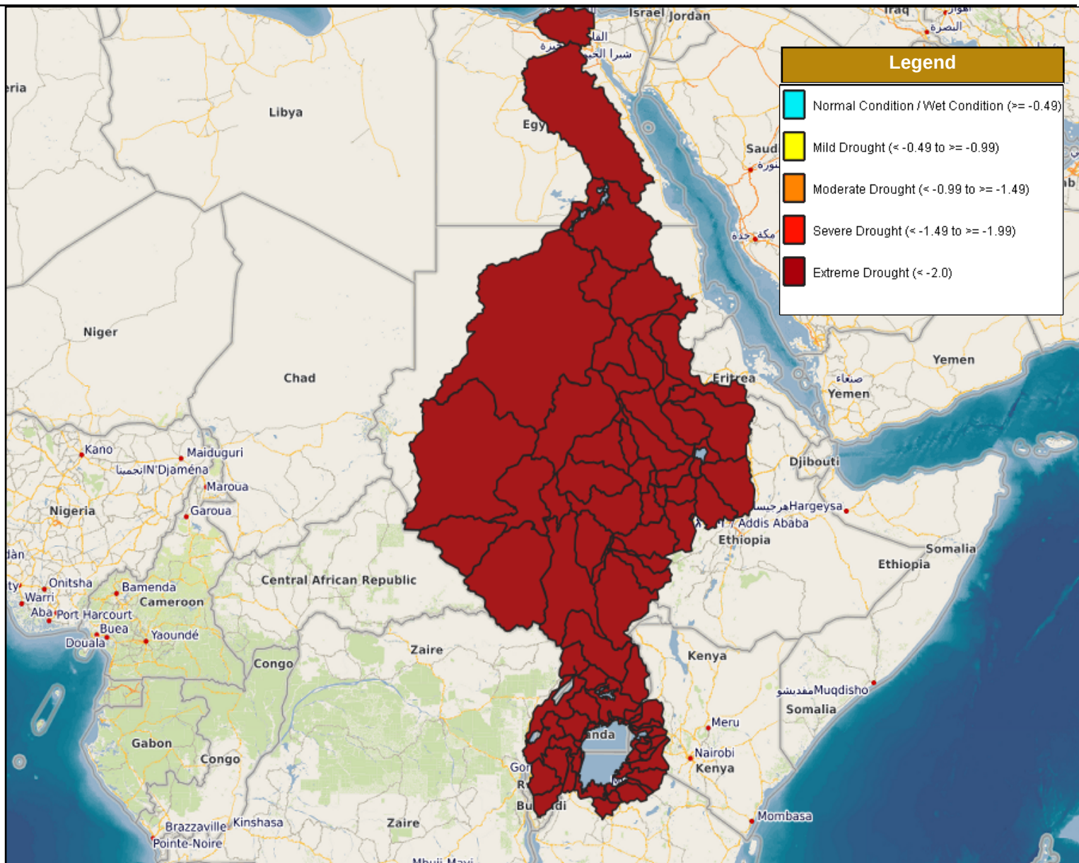
Figure 9: Spatial distribution pattern of LSTCI during the period from February-2025-April-2025
