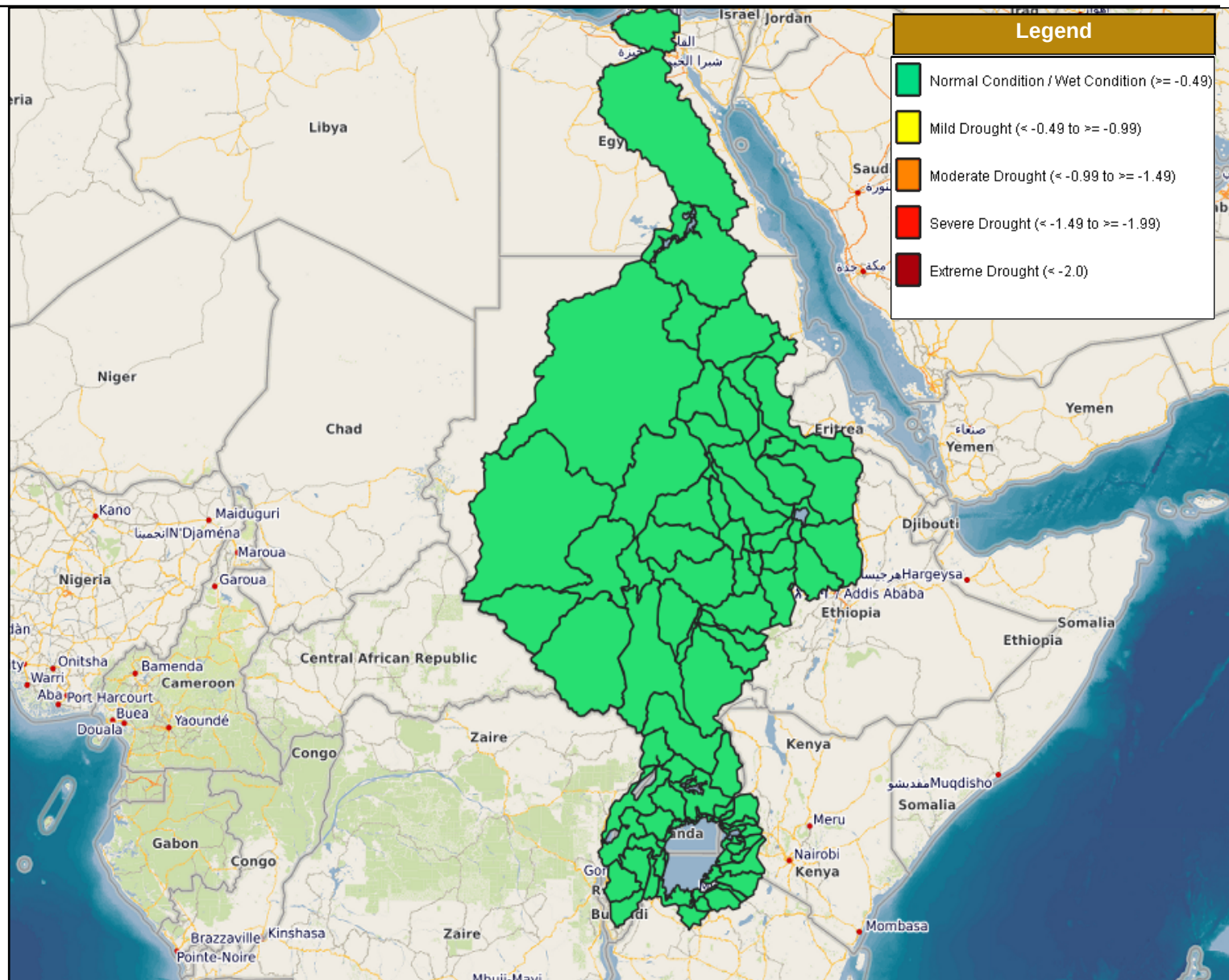
Figure 15: Spatial distribution pattern of SMAPI during the period from October-2024-March-2025
