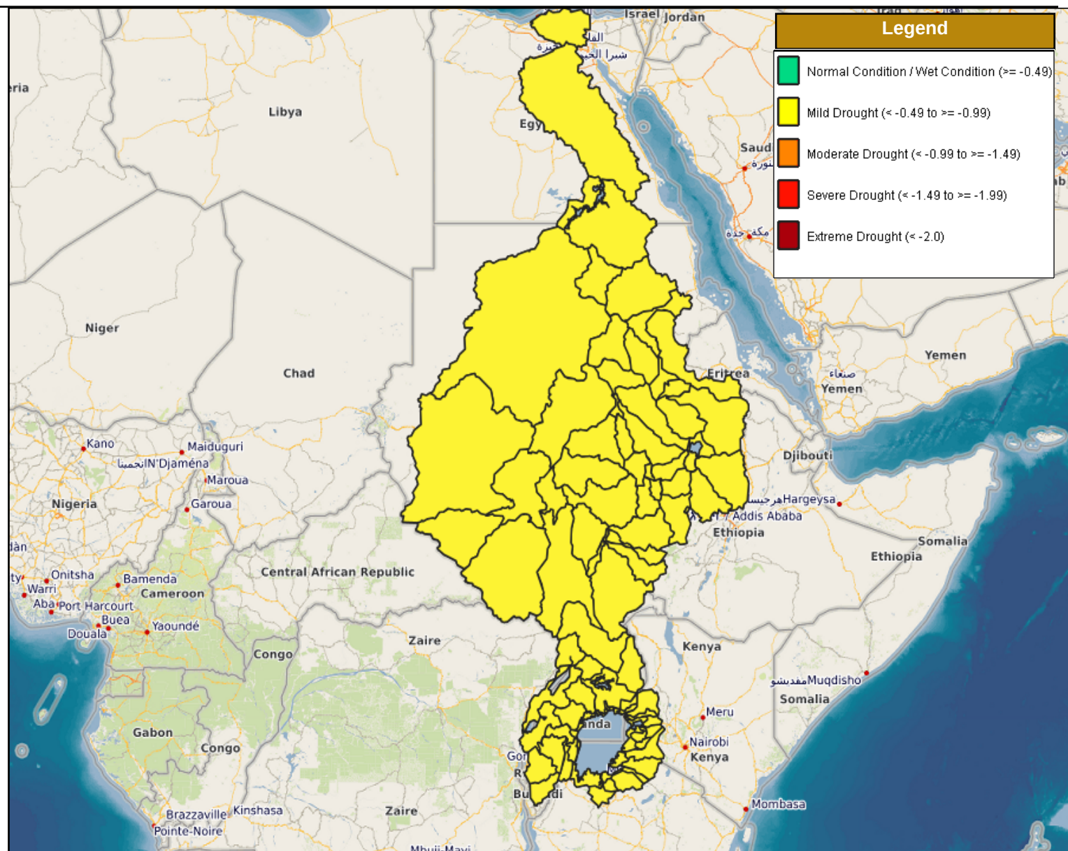
Figure 17: Spatial distribution pattern of CDI during the period from (1 - 15) Apr 2025
