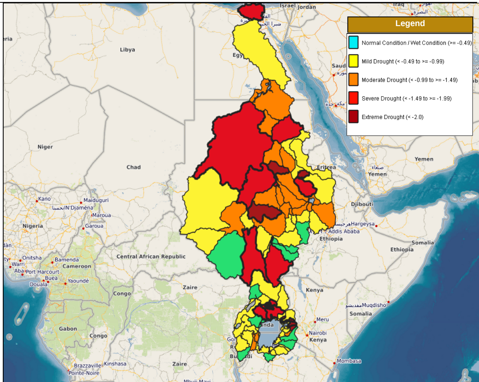
Figure 11: Spatial distribution pattern of VHI during the period from (1 - 15) Apr 2025
