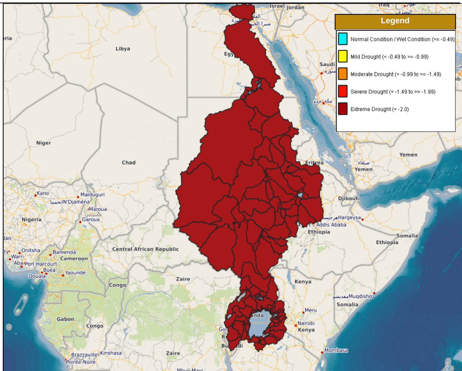
Figure 7: Spatial distribution pattern of LSTCI during the period from (16 - 30) Apr 2025
