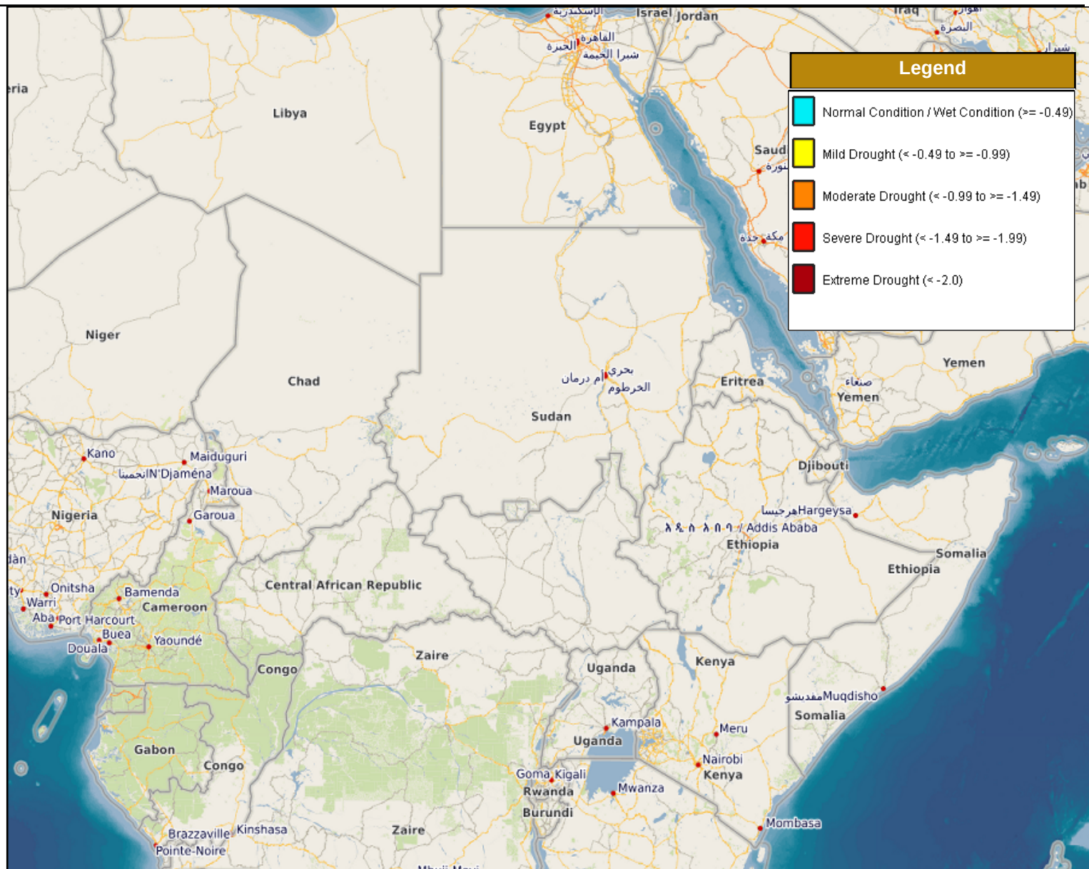
Figure 8: Spatial distribution pattern of LSTCI during the period from April 2025
