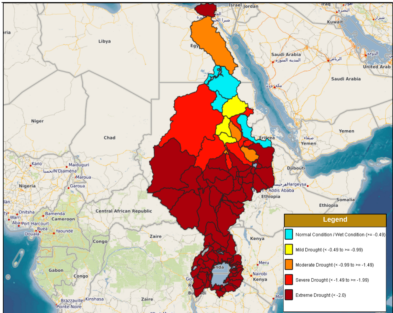
Figure 3: Spatial distribution pattern of SPI during the period from February-2025-April-2025
