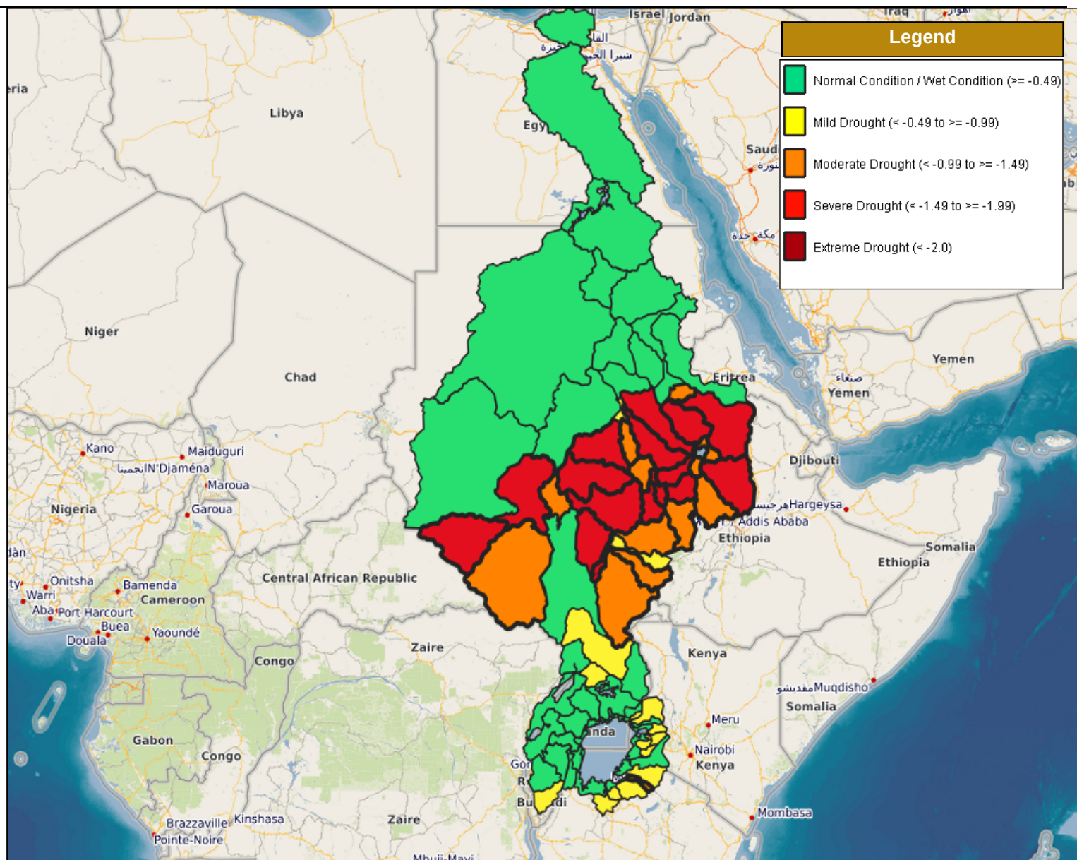
Figure 16: Spatial distribution pattern of MAI during the period from (1 - 15) Apr 2025
