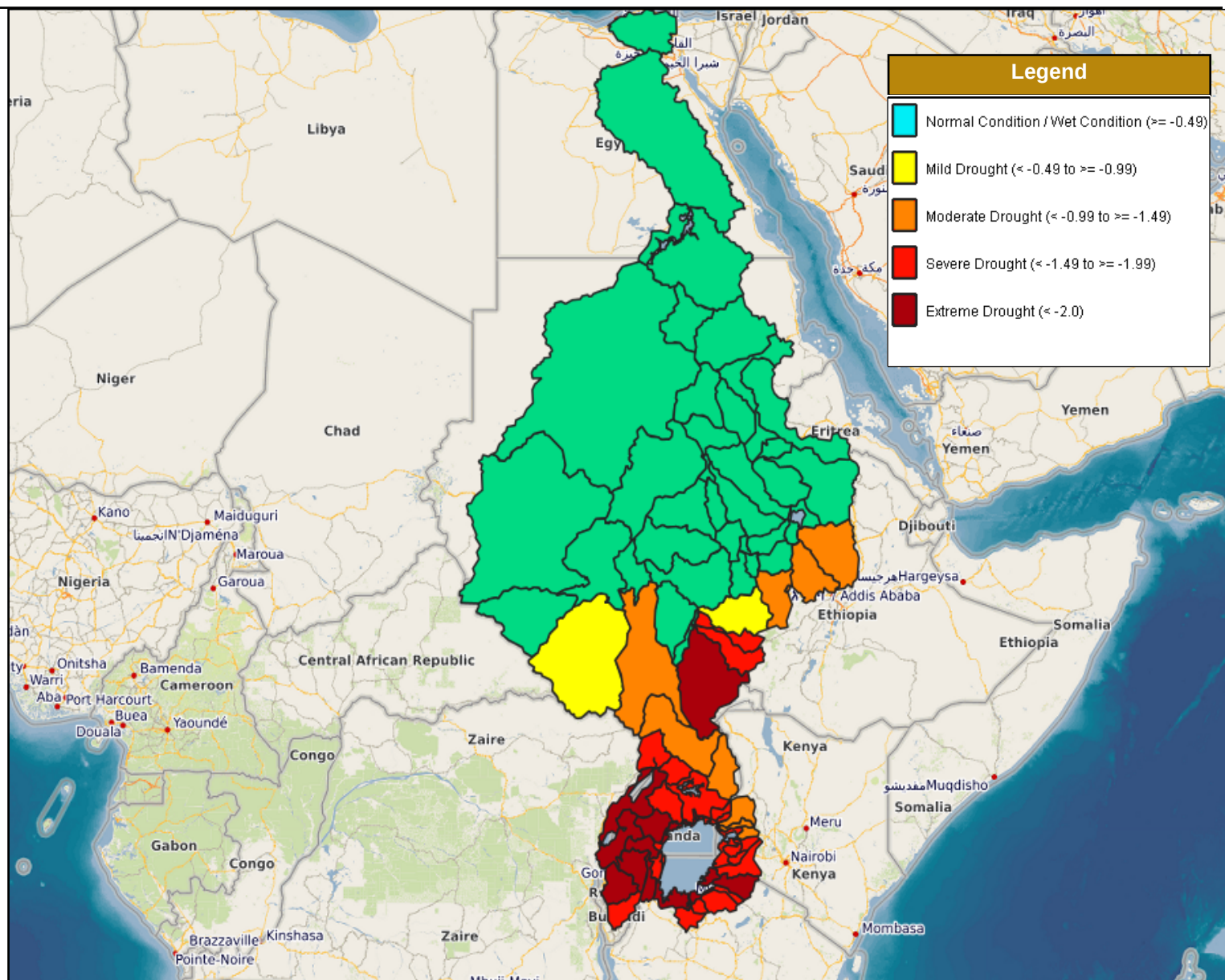
Figure 6: Spatial distribution pattern of SPEI during the period from April 2025
