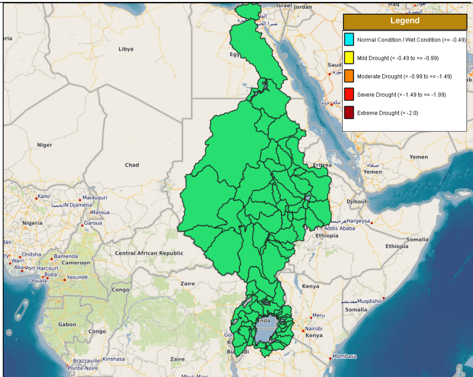
Figure 10: Spatial distribution pattern of LSTCI during the period from October-2024-March-2025
