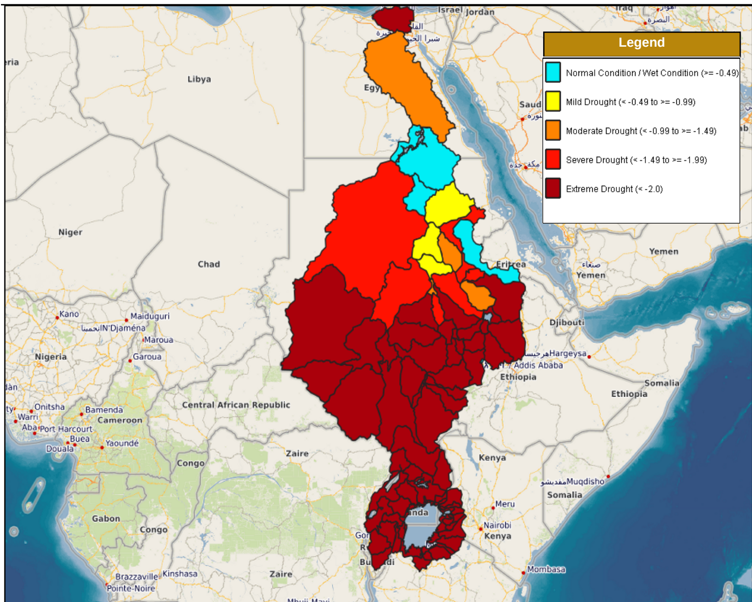
Figure 4: Spatial distribution pattern of SPI during the period from October-2024-March-2025
