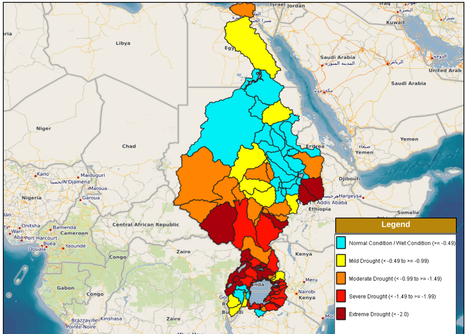
Figure 1: Spatial distribution pattern of SPI during the period from (16 - 30) Apr 2025
