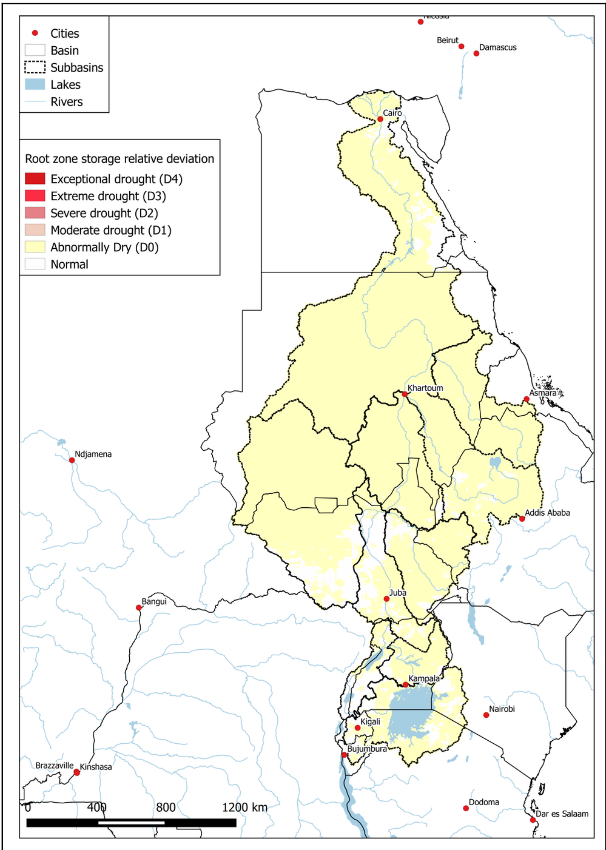
Figure 9 Map of the Root zone storage deviation for the latest 10-day period on 2024-07-01
