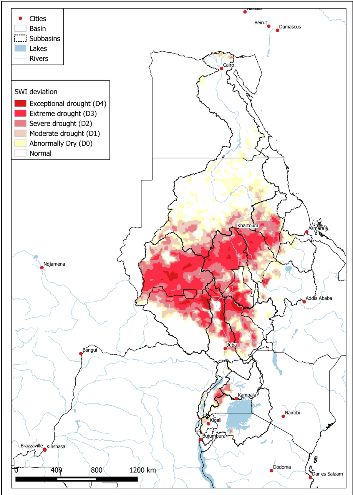
Figure 8 Map of the SWI deviation for the latest 10-day period from 2024-07-01 to 2024-07-10.
