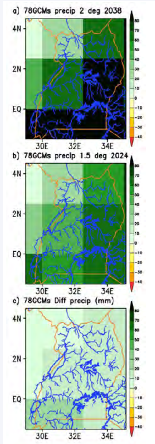
Figure 5: Projected spatial annual rainfall change for Uganda, at the time of global warming of 2°C, 1.5 °C, and the difference. Data are average from 78 CMIP5 climate model simulations under the RCP8.5 forcing scenario.
