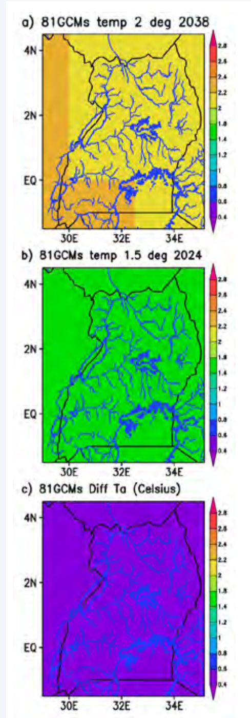
Figure 6: Projected spatial annual temperature change for Uganda, at the time of global warming level of 2°C, 1.5 °C, and the difference. Data are average from 81 CMIP5 climate model simulations under the RCP8.5 forcing scenario.
