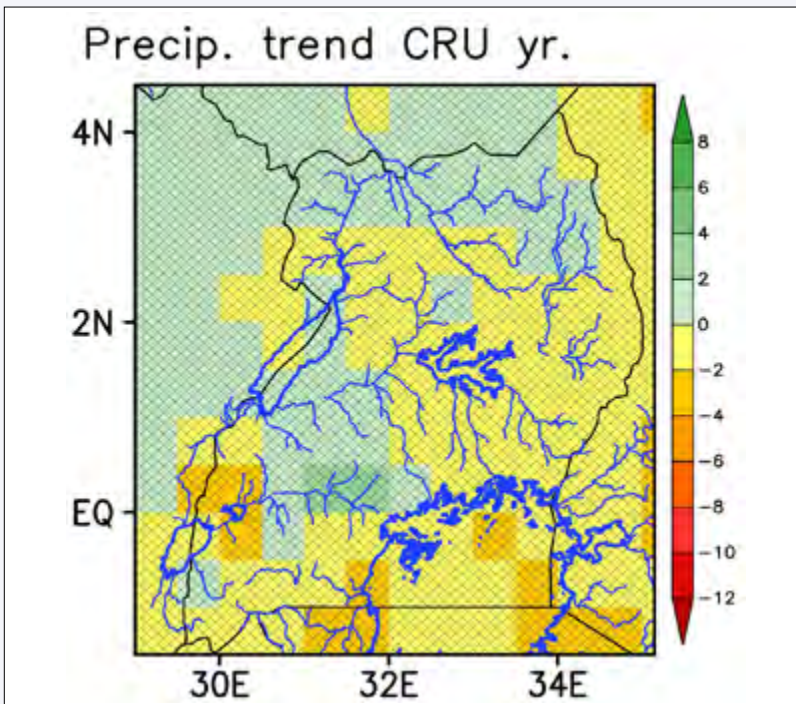
Figure 3: The monotonic slope in precipitation (mm) between 1963 and 2012 at each grid cell, according to a linear trend per decade for Jan. to Dec. Hatching indicates areas where the trend is not statistically significant at the 95% level. Data taken from the CRU TS3.22 datasets.
