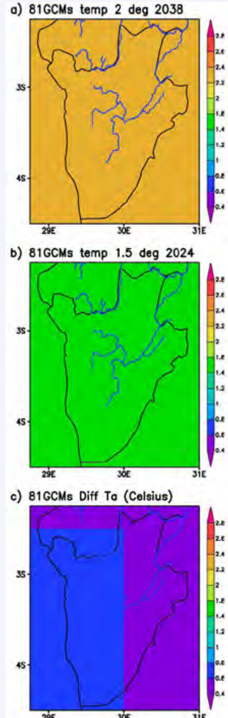
Figure 6: Projected spatial annual temperature change for Burundi, at the time of global warming of 2°C, 1.5 °C, and the difference. Data are average from 81 CMIP5 climate model simulations under the RCP8.5 forcing scenario.
