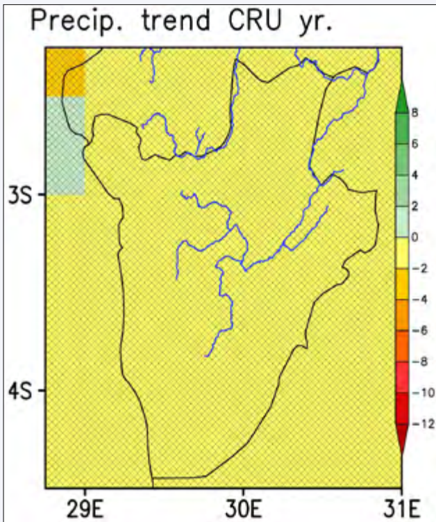
Figure 3: The monotonic slope in precipitation (mm) between 1963 and 2012 at each grid cell, according to a linear trend per decade for Jan. to Dec. Hatching indicates areas where the trend is not statistically significant at the 95% level. Data taken from the CRU TS3.22 datasets.
