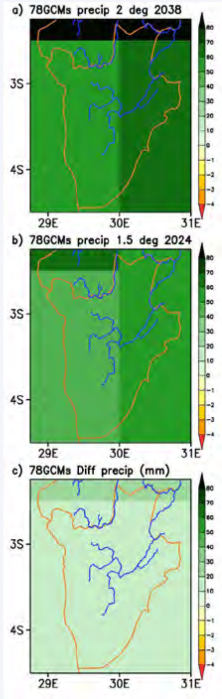
Figure 5: Projected spatial annual rainfall change for Burundi, at the time of global warming of 2°C, 1.5 °C, and the difference. Data are average from 78 CMIP5 climate model simulations under the RCP8.5 forcing scenario.
